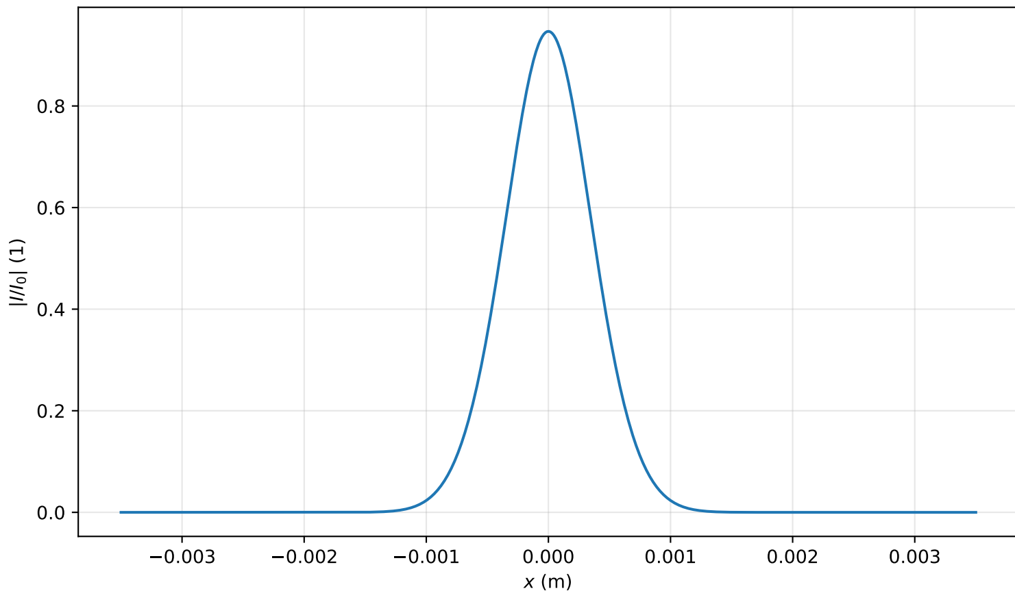
Intensity profile I(x, y = 0, z = 0.716m)/I_0 , P_{in}=0.2P_{cr} , artificial time
